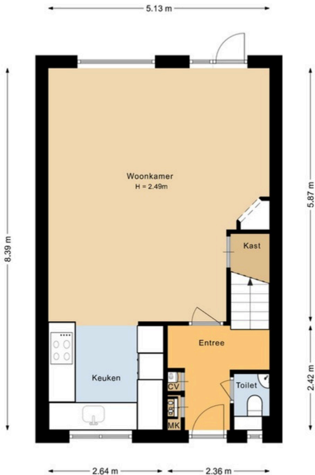
Walakker 119 Purmerend Begane Grond
