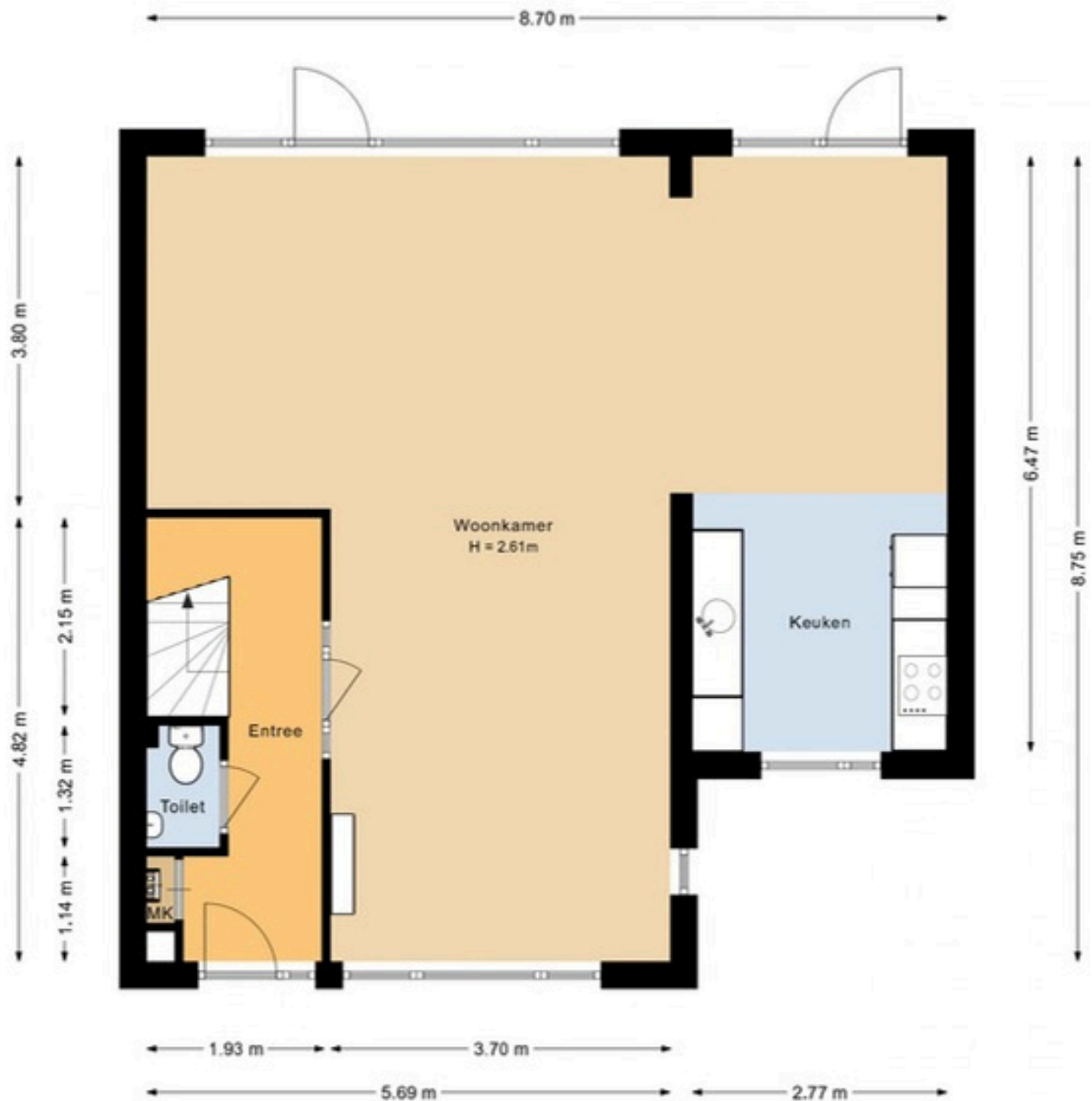
Borghesepark 5 Purmerend Begane grond
