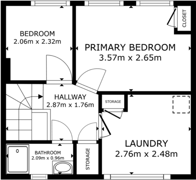
FLOOR 2
