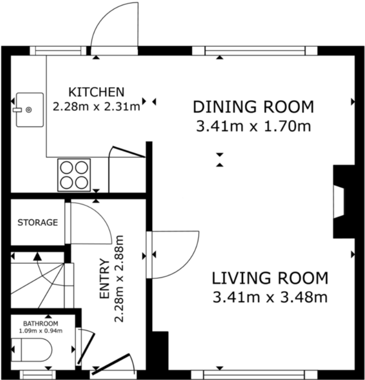
FLOOR 1
