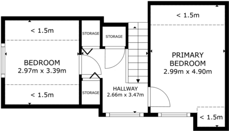
FLOOR 2
