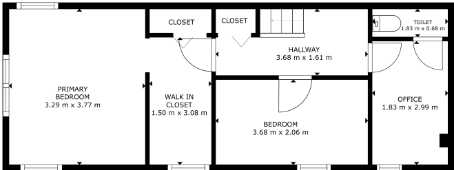
FLOOR 2
