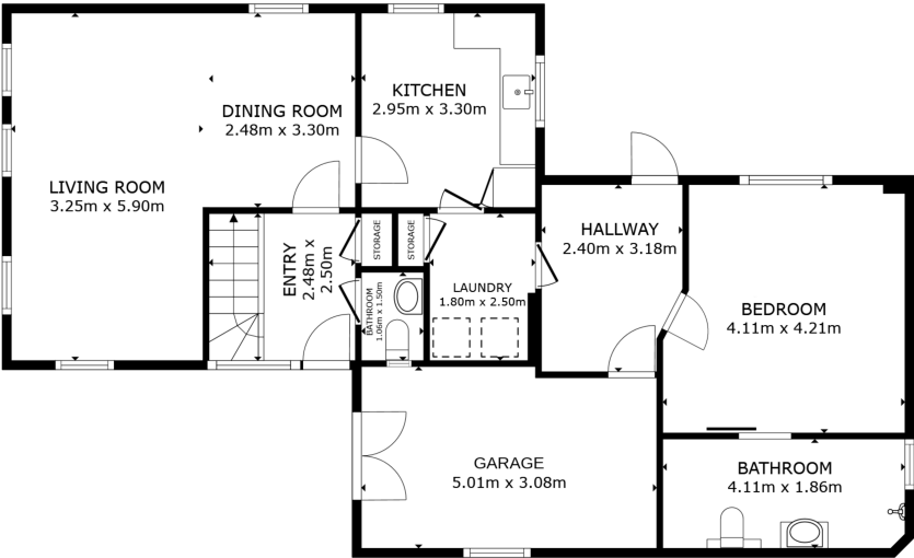
FLOOR 1
