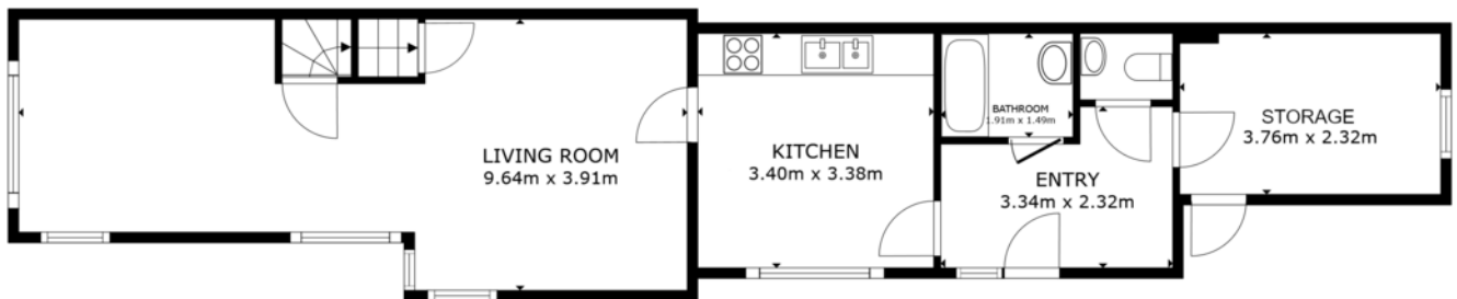
FLOOR 1
