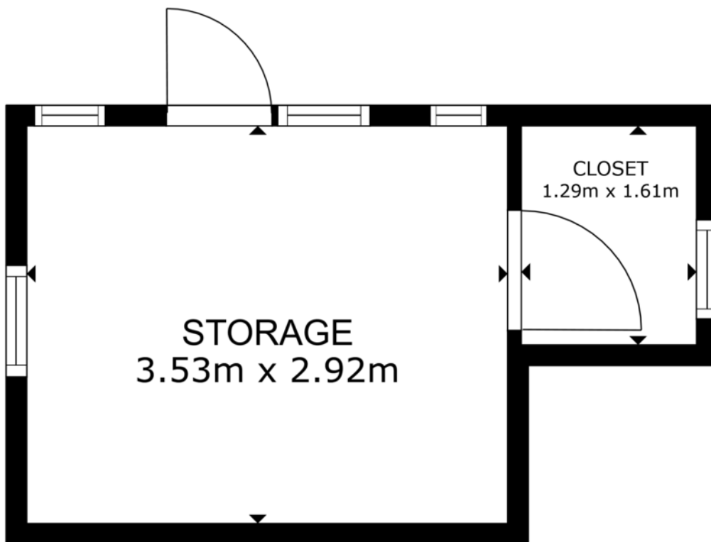
FLOOR PLAN
