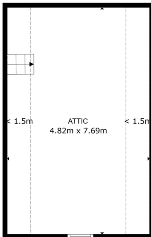
FLOOR PLAN
