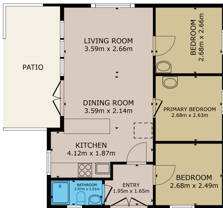
FLOOR PLAN
