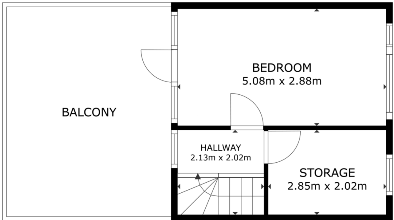
FLOOR 3
