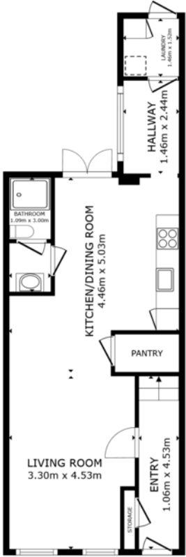
FLOOR 1
