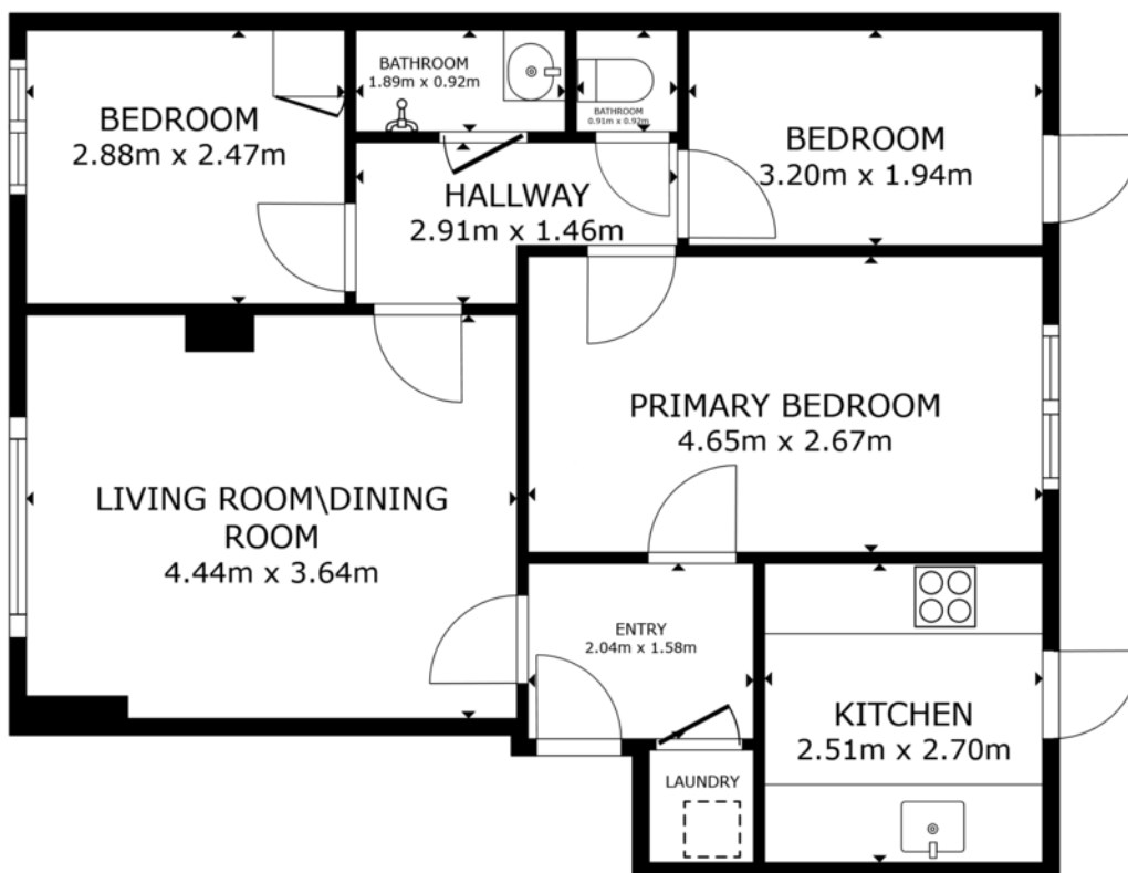
FLOOR PLAN
