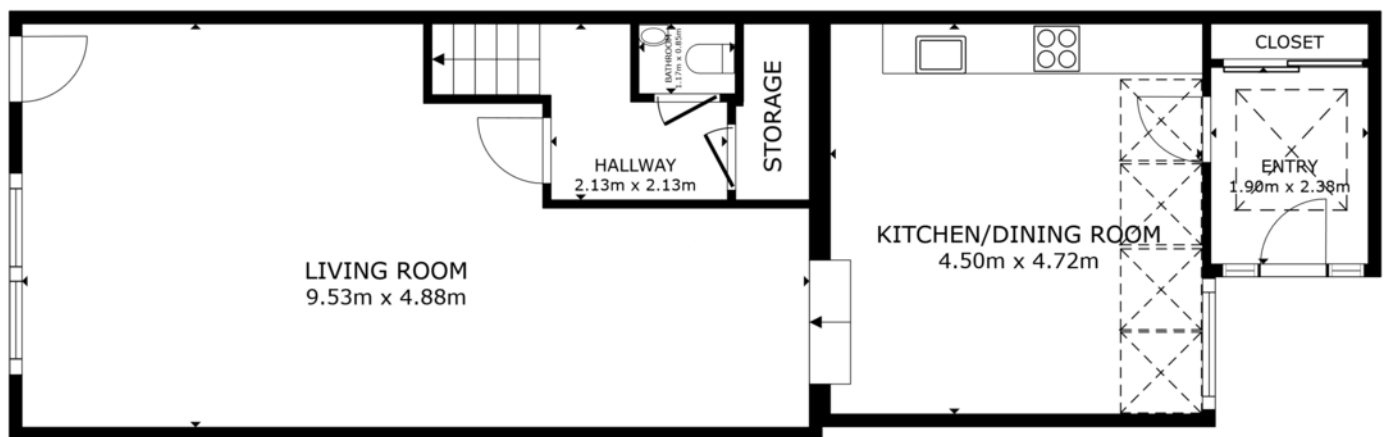
FLOOR 1
