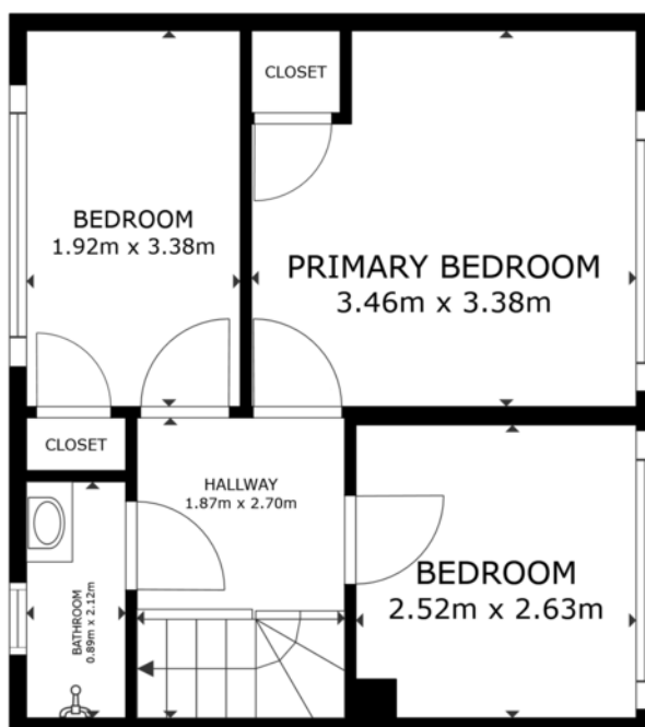
FLOOR 2
