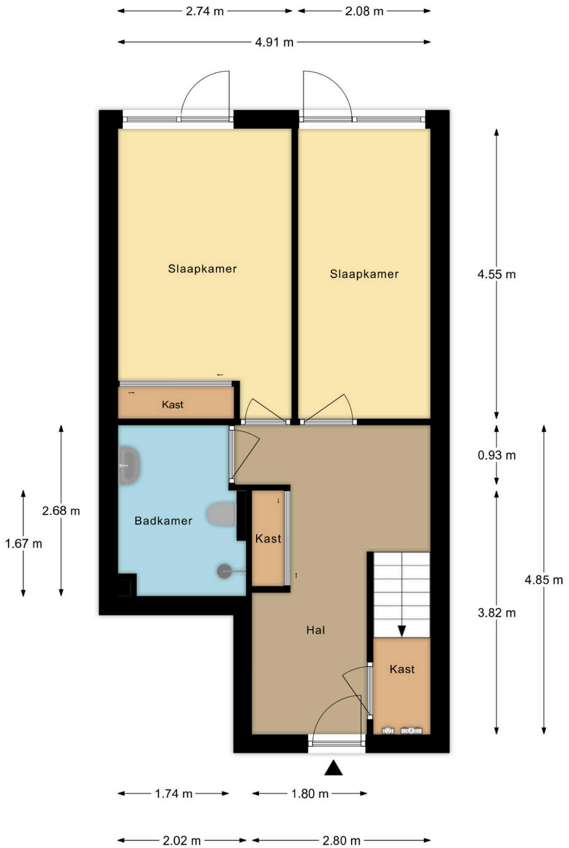
Engelenburg 188 Haarlem Begane Grond
