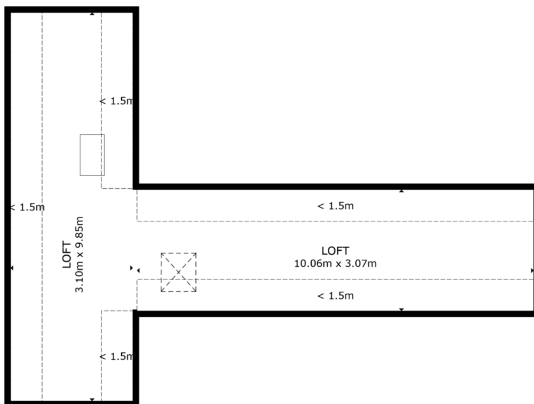
FLOOR PLAN
