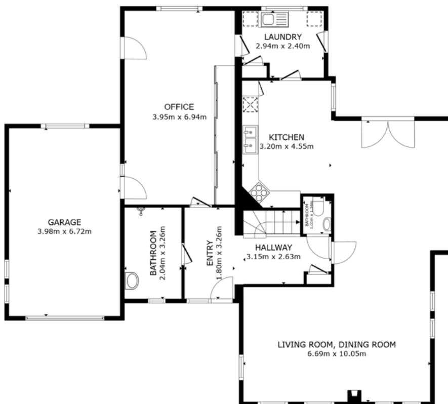
FLOOR 1
