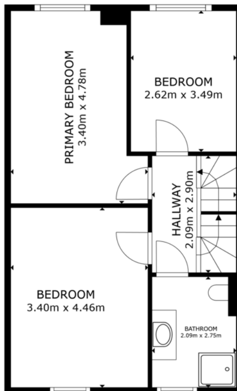
FLOOR 2
