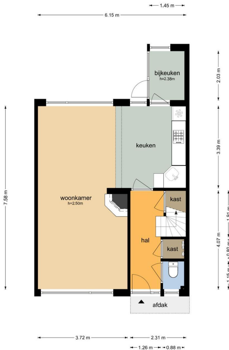
Aalsburg 2211 - Wijchen Begane Grond
