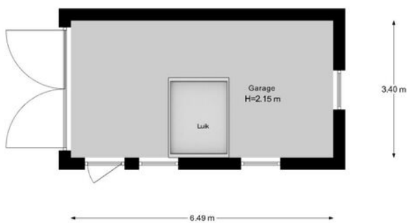
Garage Begane Grond
