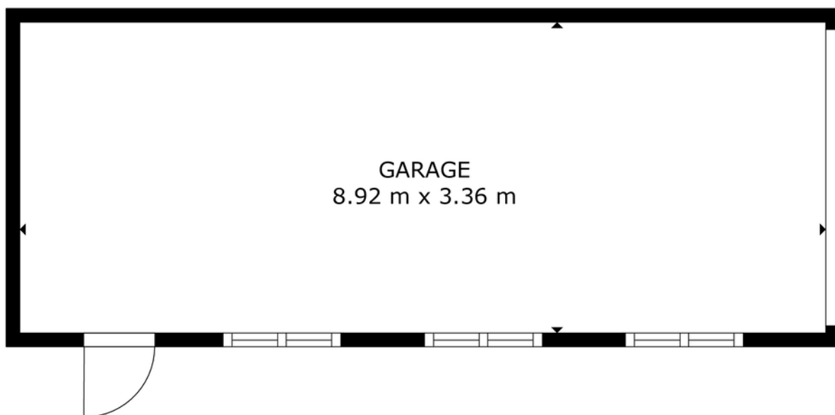
FLOOR PLAN
