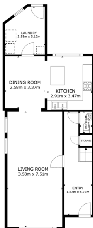
FLOOR 1
