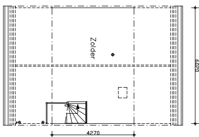
Zolder
