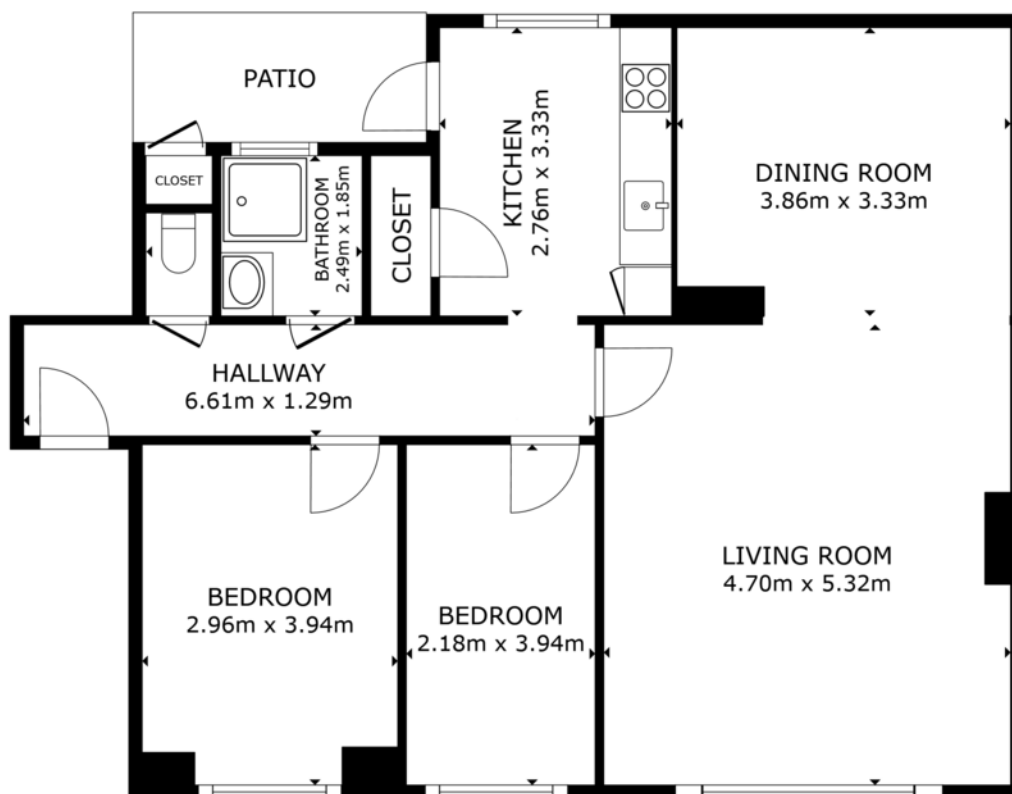
FLOOR PLAN
