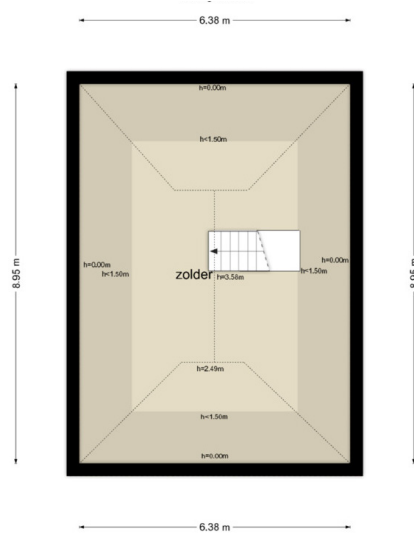
Garage zolder
