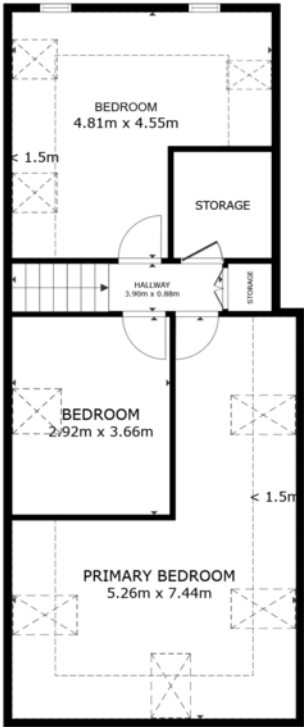
FLOOR 2
