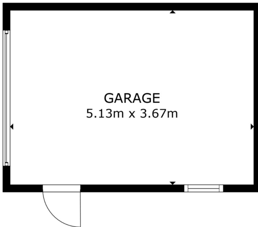
FLOOR PLAN
