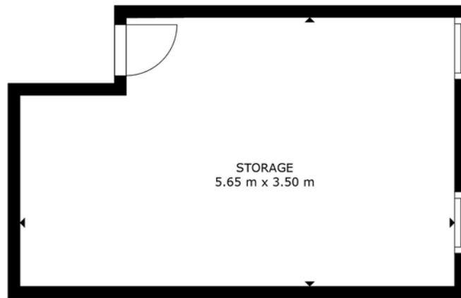
FLOOR PLAN
