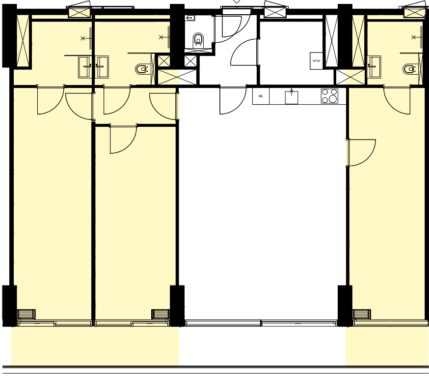
LOFT 150M 2 (60M 2 +3x30M 2 )
