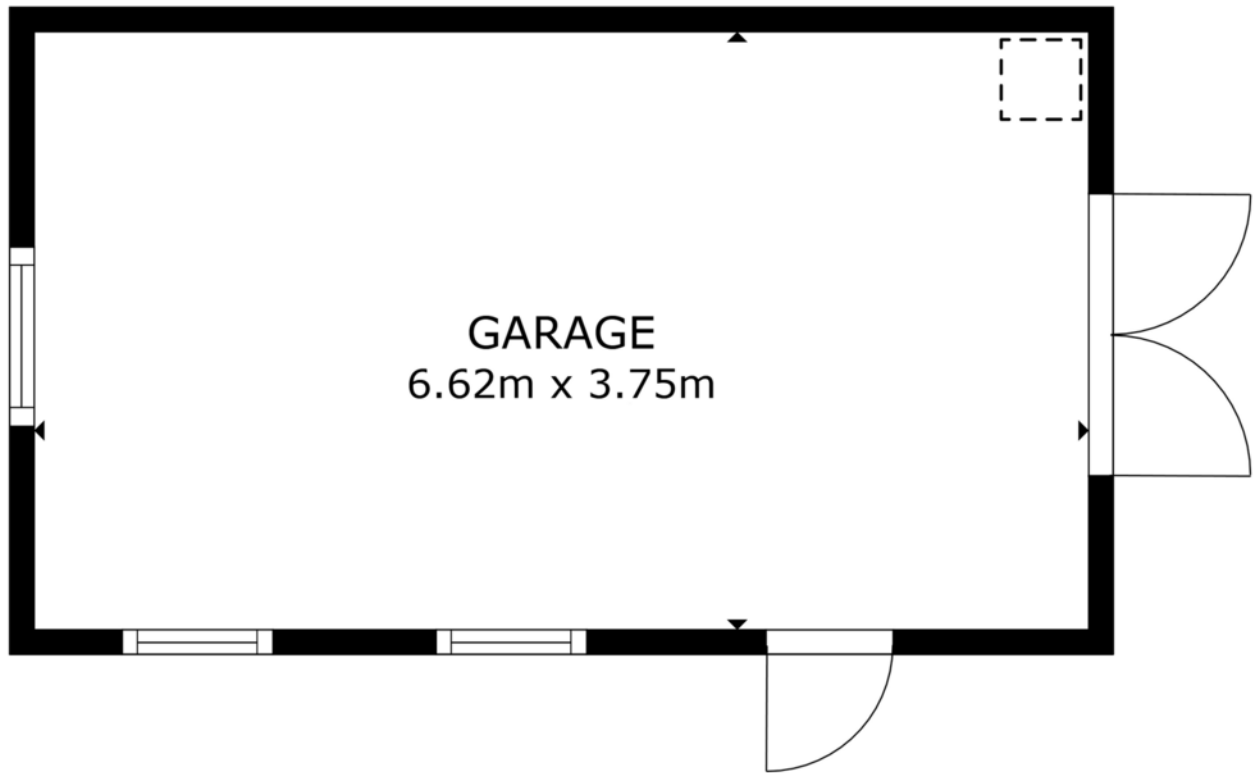
FLOOR PLAN
