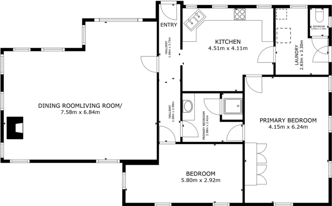
FLOOR PLAN
