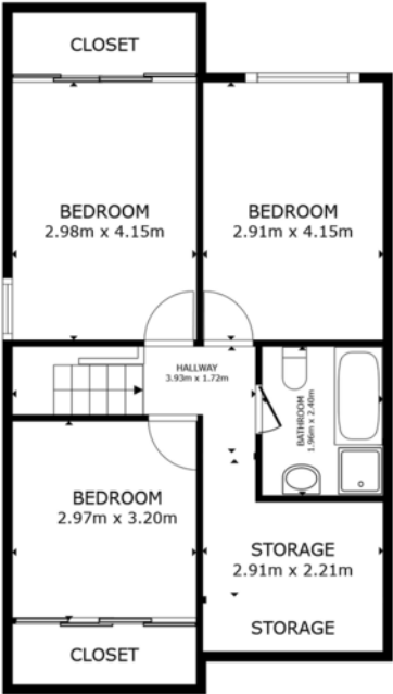
FLOOR 2
