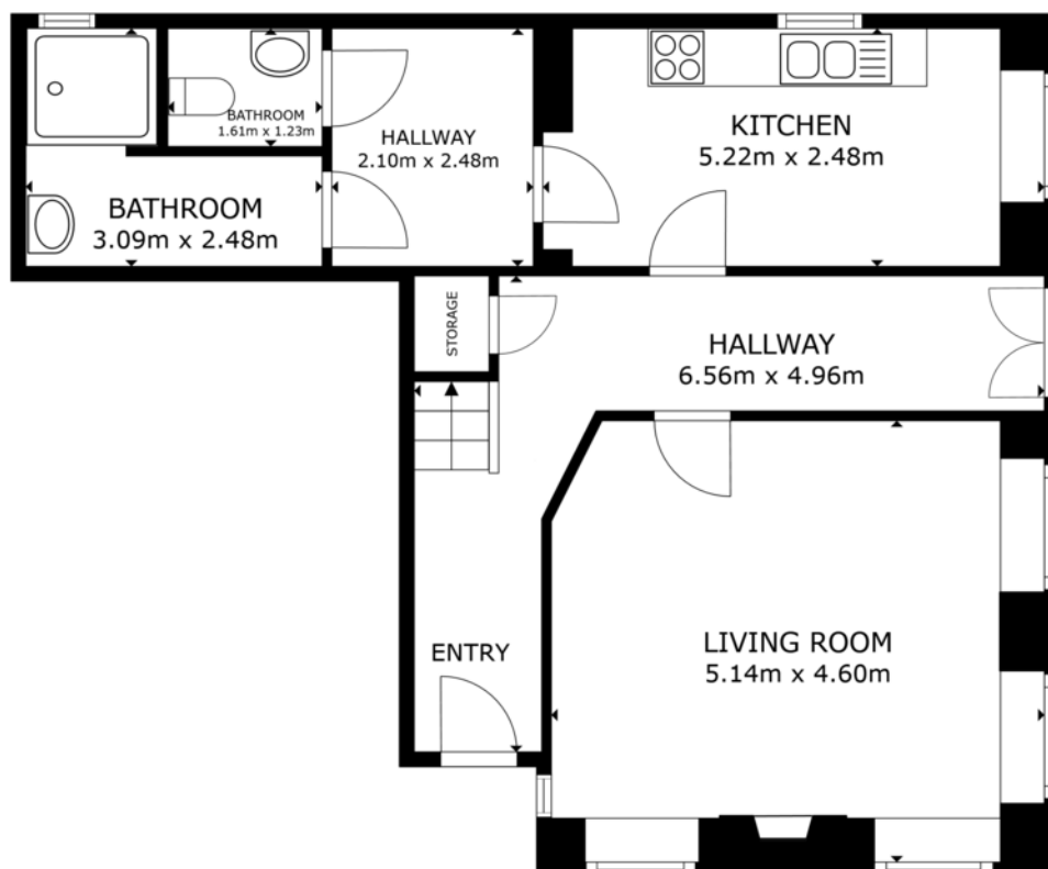
FLOOR 1
