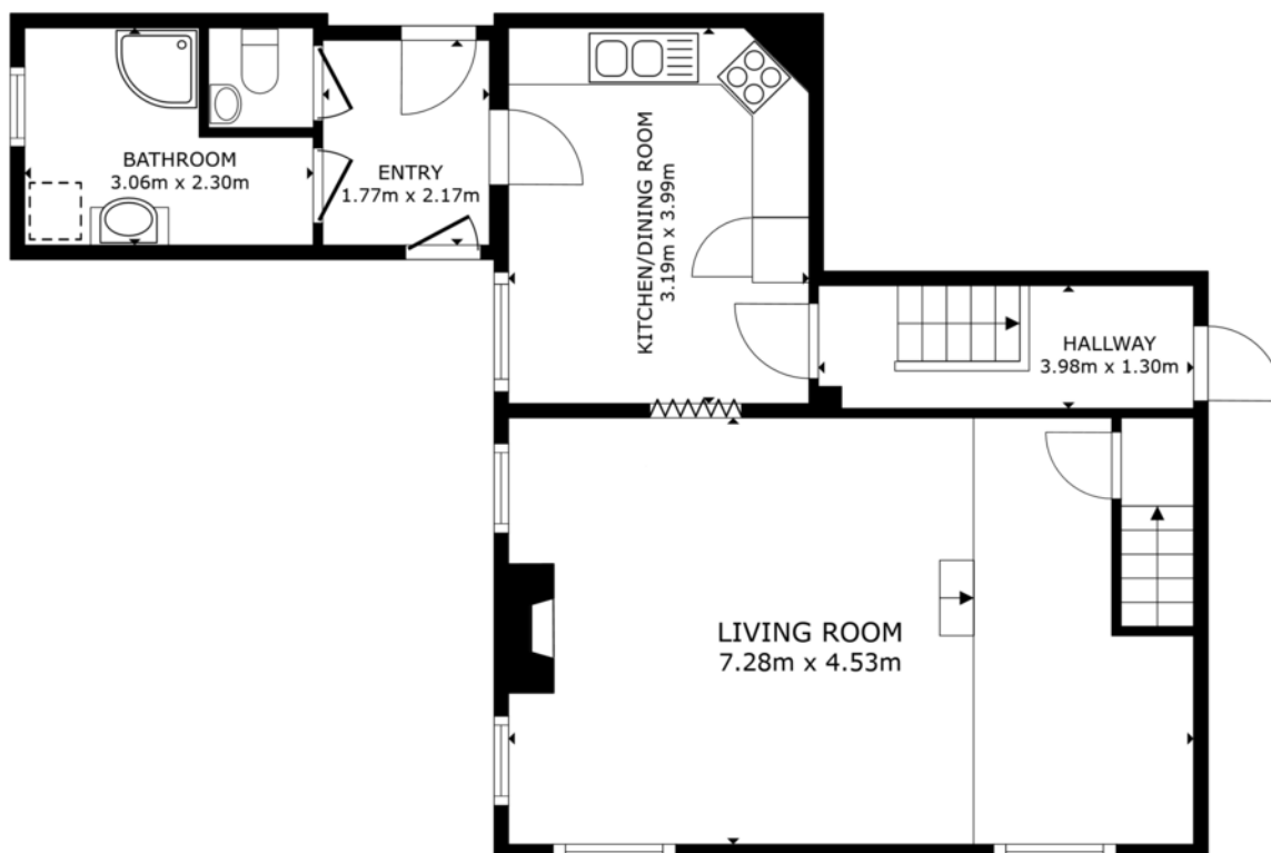
FLOOR 2
