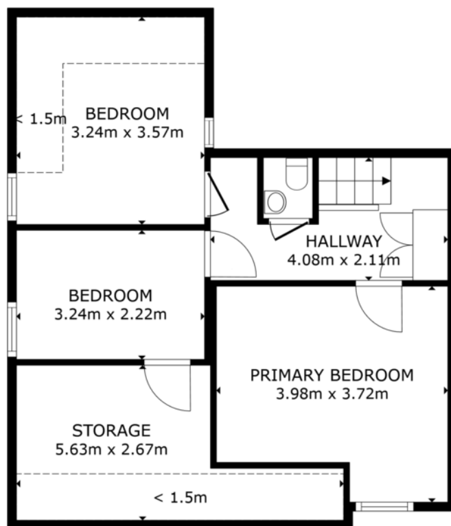
FLOOR 3
