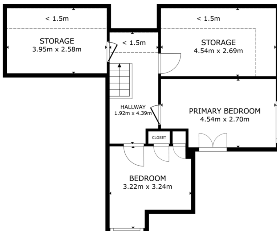
FLOOR 2
