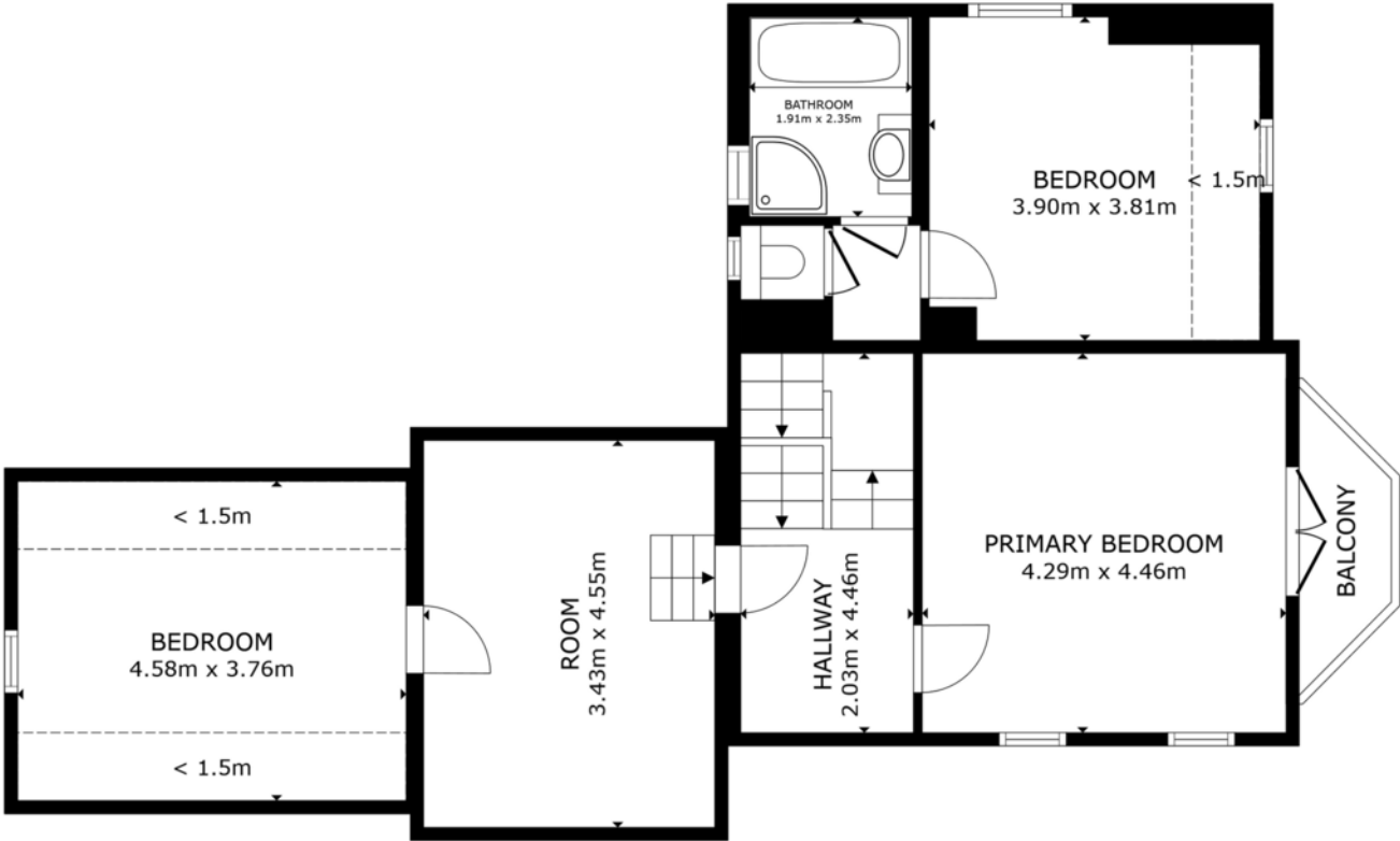
FLOOR 2
