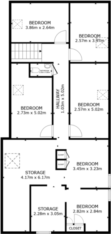
FLOOR 2
